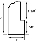
ATLANTA FLAT AFL
