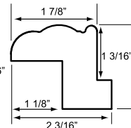
MALIBU Z-FRAME MAZ
