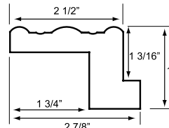
MEDIUM Z-FRAME MDZ
