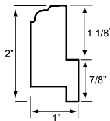
ATLANTA Z-FRAME AZF
