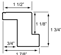
SINGLE BEADED Z-FRAME SBZ
