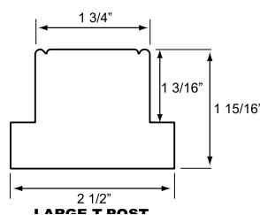
LARGE T POST
