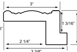
LARGE Z-FRAME LGZ
